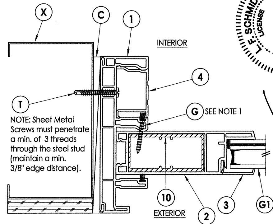
5 HORIZONTAL CROSS SECTION
