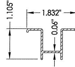
15 ANTI-LIFT-OUT BLOCKS 8567-356-D54
